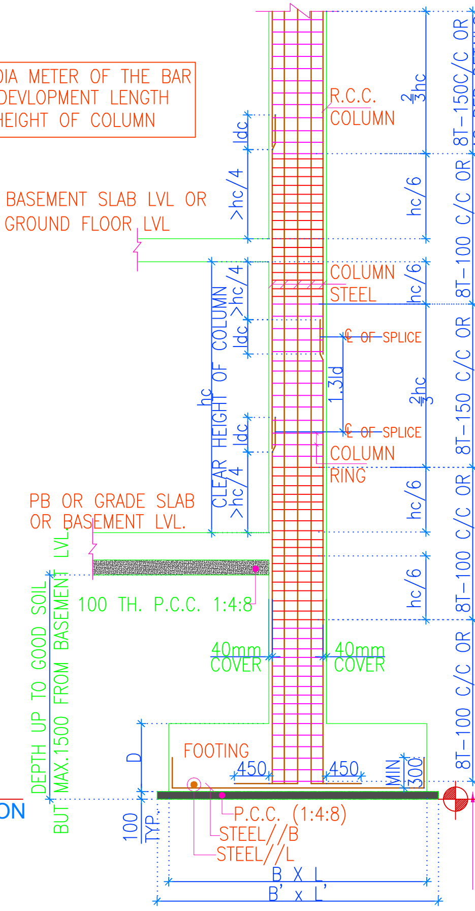
TYPICAL COLUMN FOOTING SECTION: X-X (DUCTILITY DETAIL FOR COLUMN) (LAPPING OF VERTICAL BARS)
